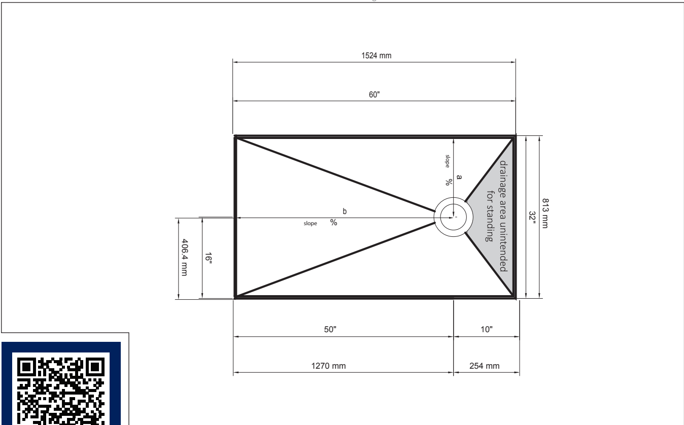
Technical Drawing
