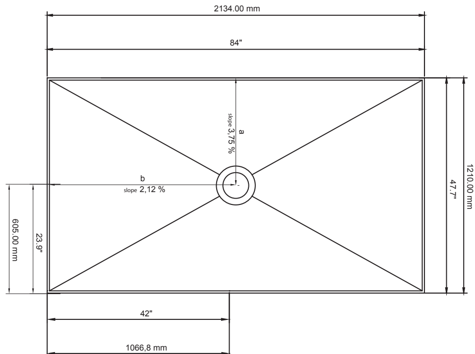
Technical Drawing
