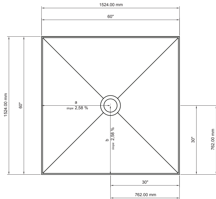
Technical Drawing
